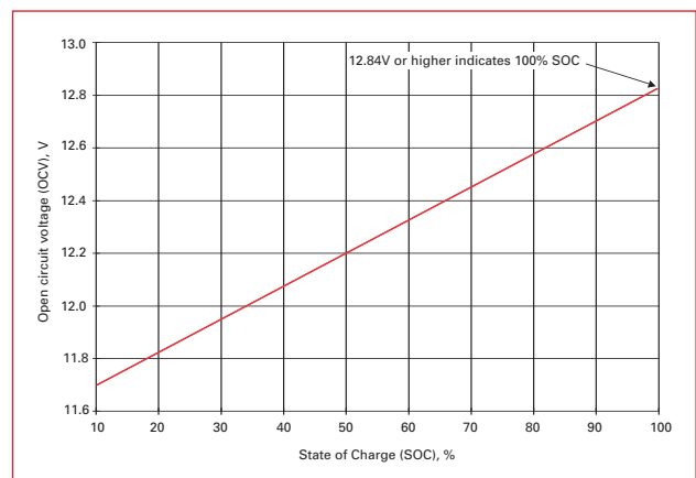
Figure 2: Open circuit voltage and state of charge
