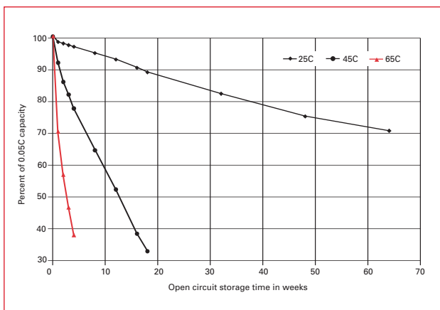
Figure 3: ODYSSEY storage time at temperatures
