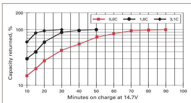
Figure 7: Quick charging ODYSSEY batteries
