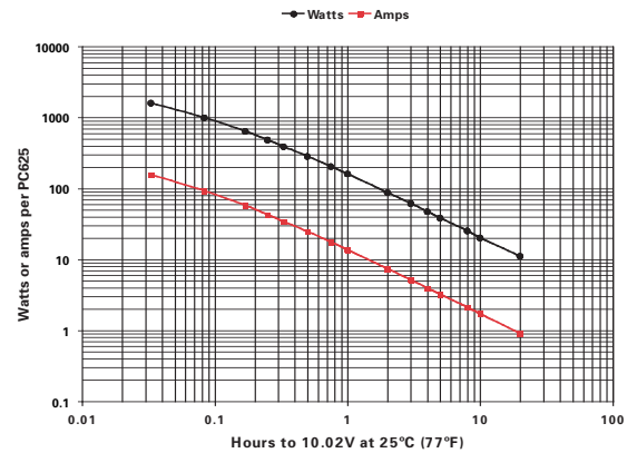
PC625 performance data at 25°C, per 12V module
