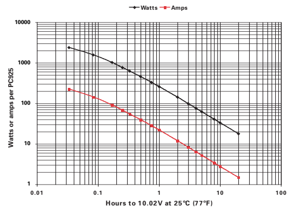
PC925 performance data at 25°C, per 12V module
