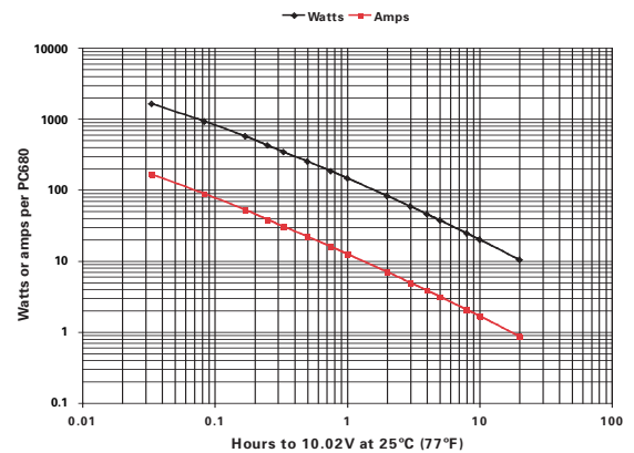
PC680 performance data at 25°C, per 12V module
