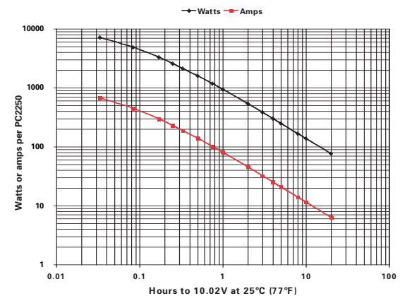
PC2250 performance data at 25°C, per 12V module
