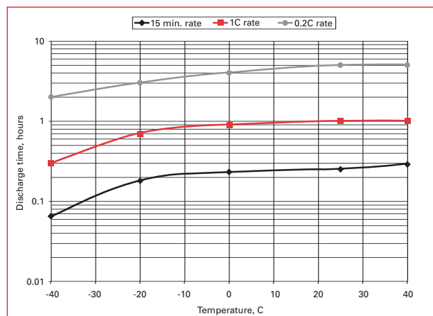
Figure 5: ODYSSEY capacity at temperatures
