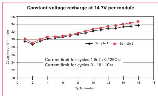
Figure 4: Recovery from high temperature discharged storage
