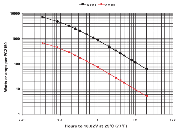
PC2150 performance data at 25°C, per 12V module
