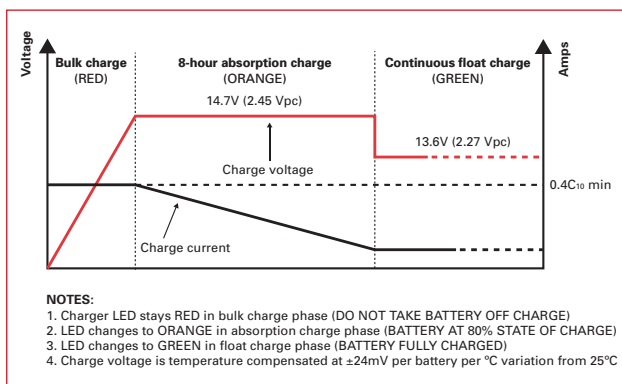
Figure 6: Recommended three-step charge profile
