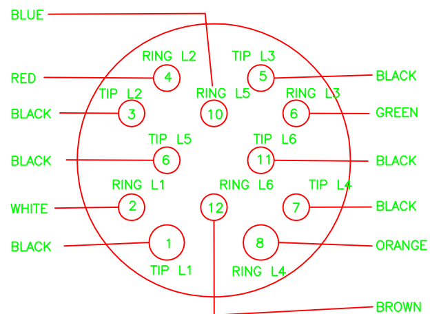
SECTION A-A (SEE NOTE 4) (REAR VIEW)
