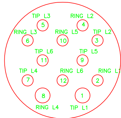
SECTION B-B (SEE NOTE 4) (REAR VIEW)
